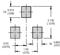
RECOMMENDED FOOTPRINT
